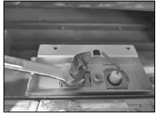
Figure 24: Adjust shutter.
