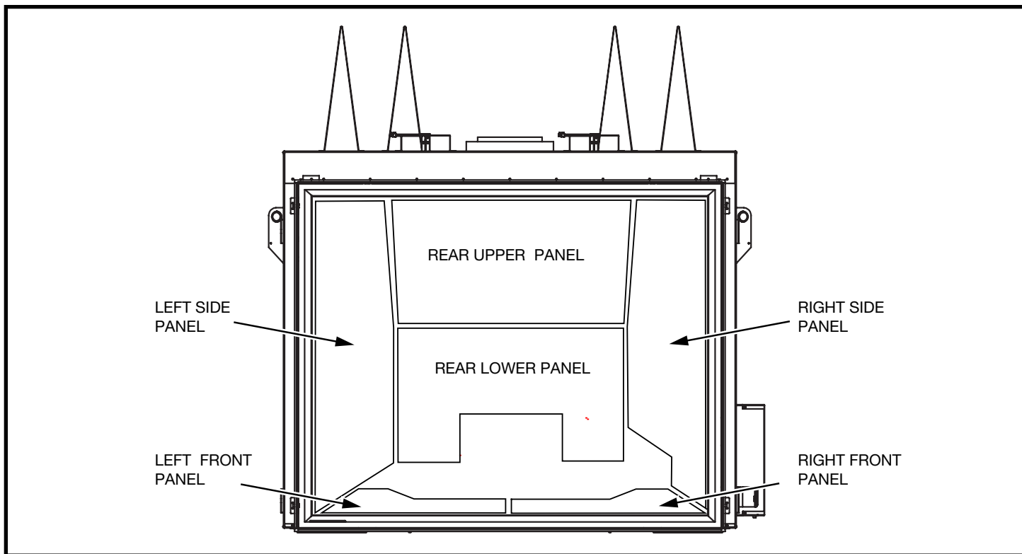
Figure 50: Panel locations.
