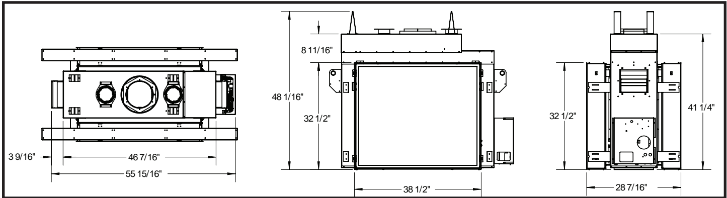
Figure 1: TC36ST Overall dimensions.
