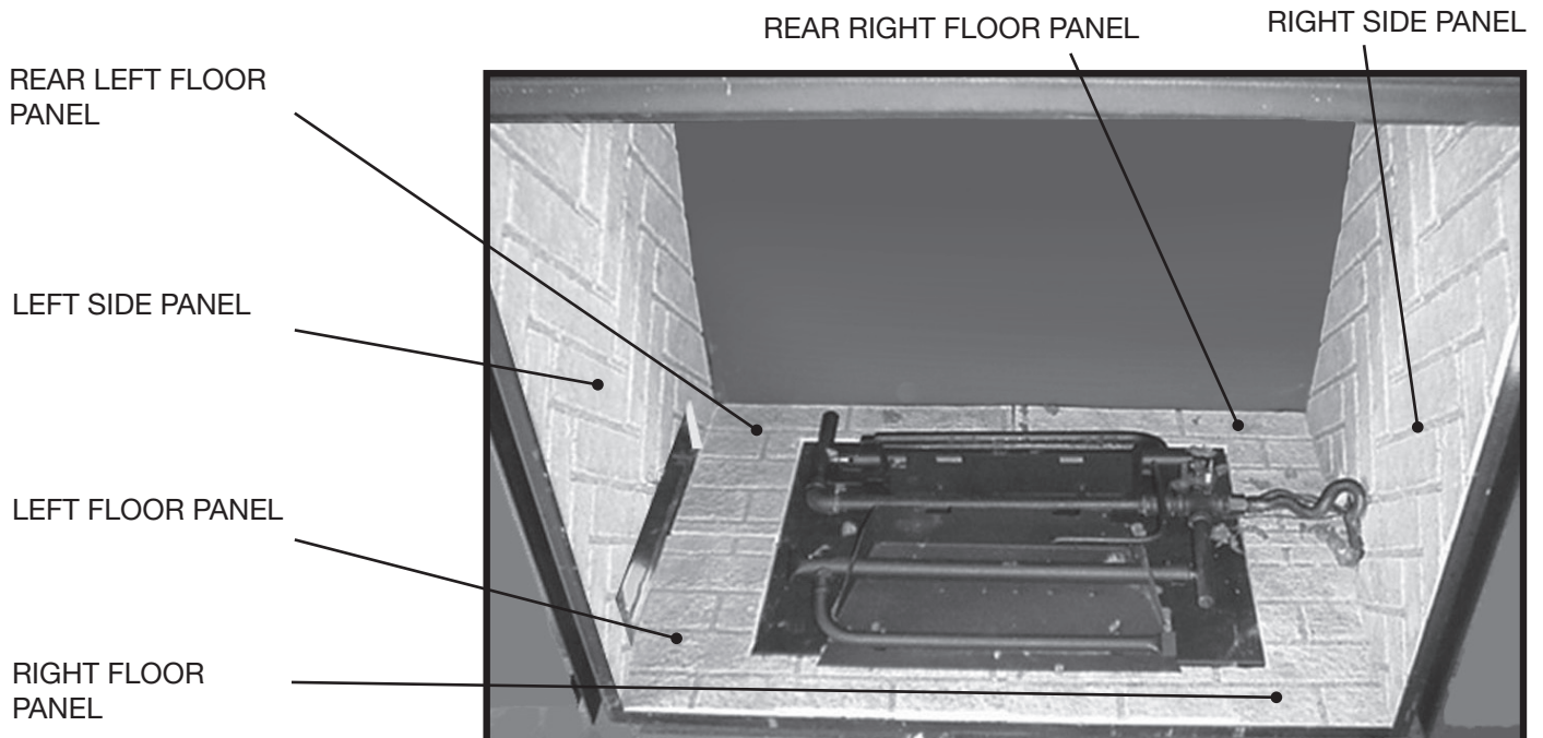
Figure 52: TC36ST Panels.
