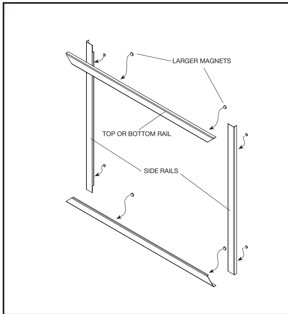
Figure 53: TC36ST Trim kit.
