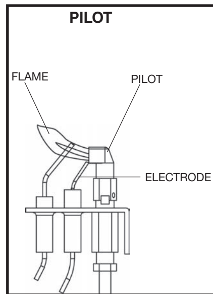
Figure 54: Pilot assembly.
