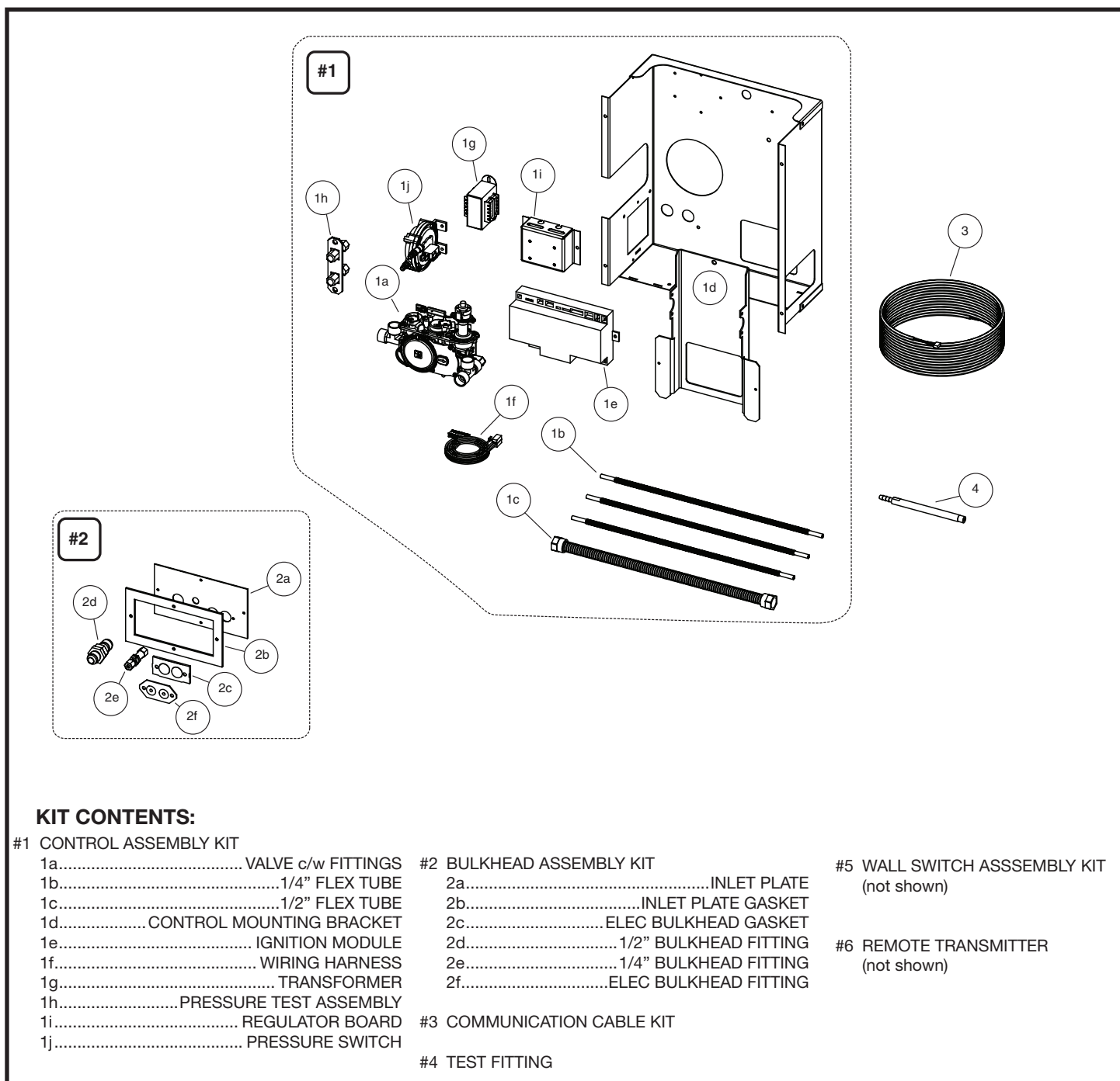
Figure 56: TC36ST Control system.
