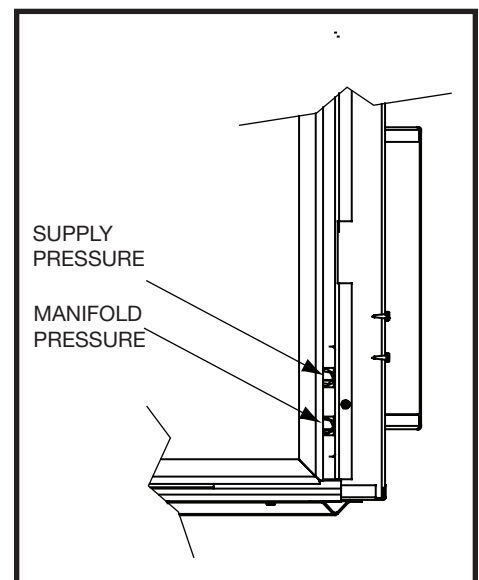
Figure 33: Test ports.
