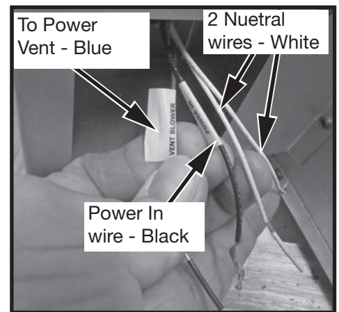
Figure 25: Junction box wiring.
