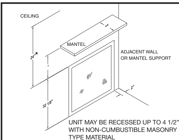
Figure 3: TC36ST Mantel.
