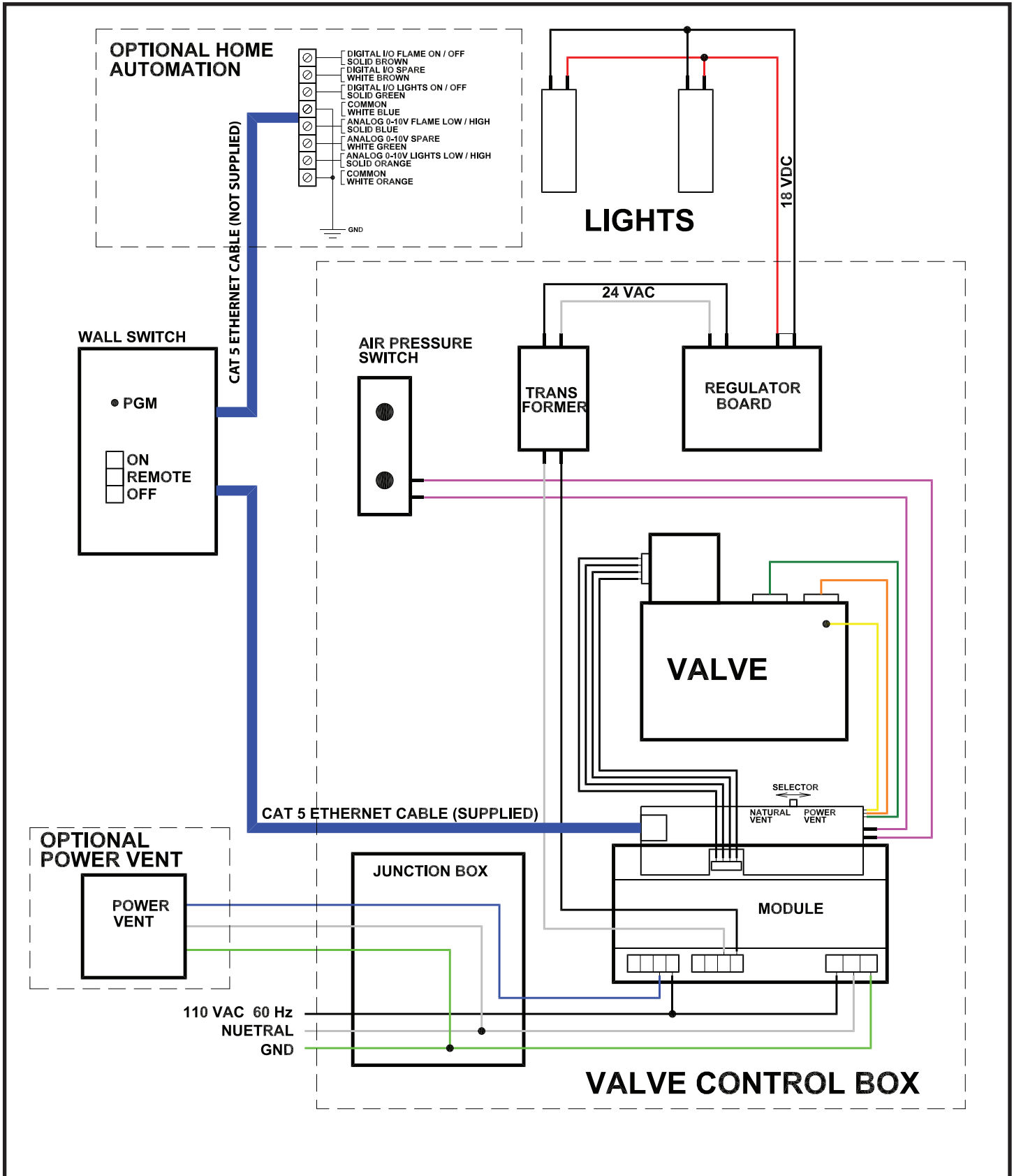
Figure 57: TC36ST Wiring diagram.
