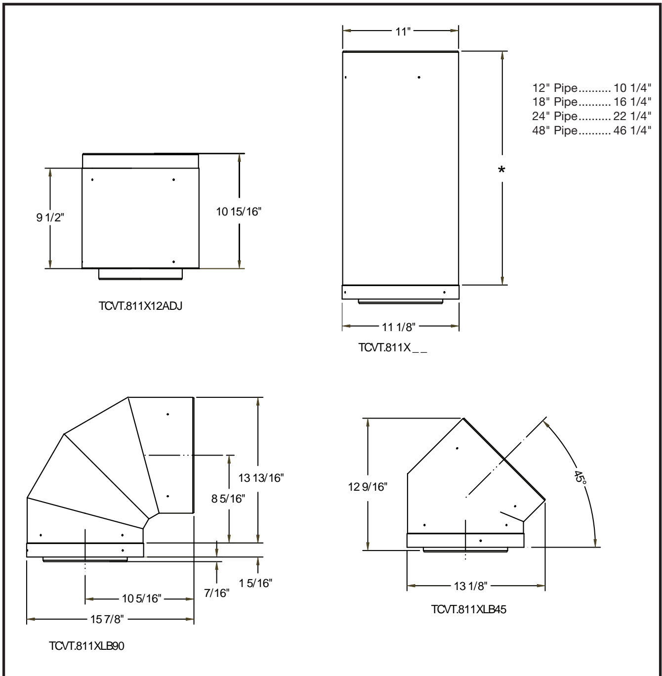
Figure 50: Vent pipe dimensions.
