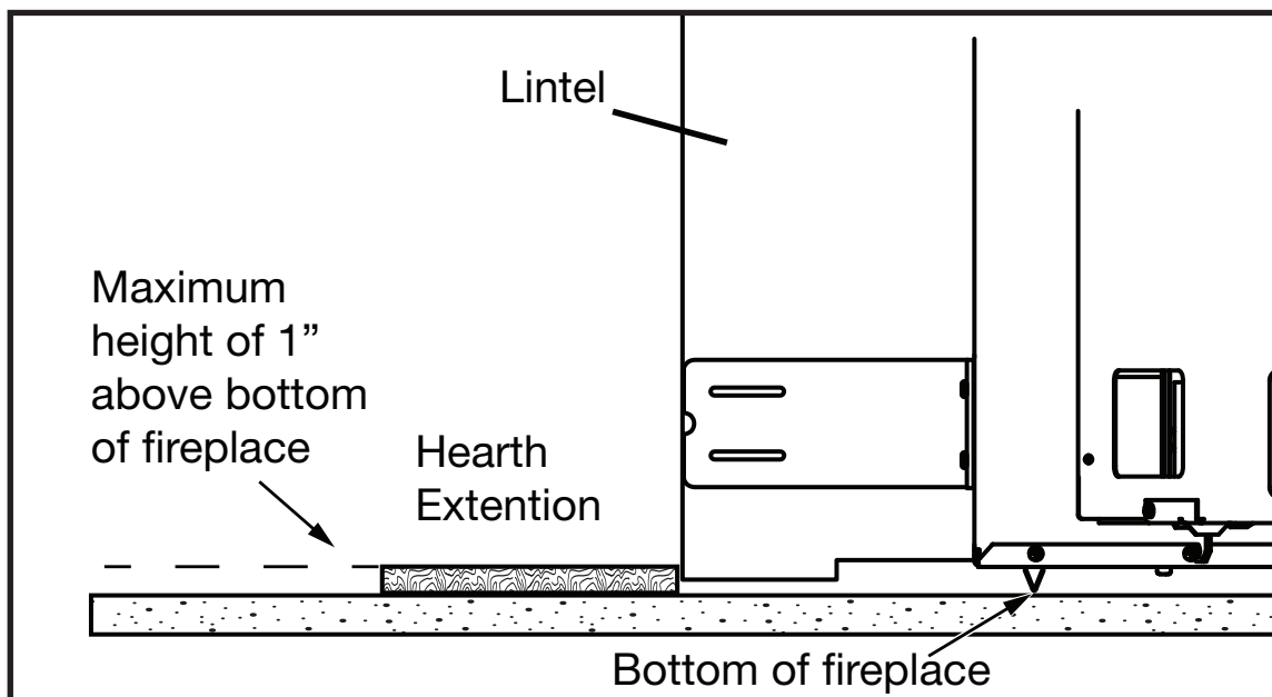
Figure 23: Hearth extension.
